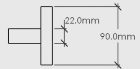
ELEVATION - SIDE
