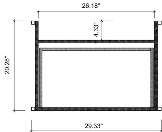
DRAWER PLAN DETAIL
