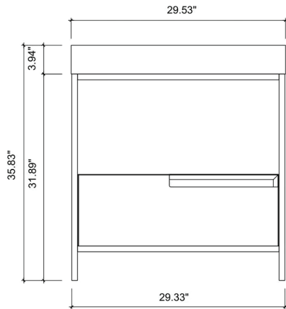
FRONT ELEVATION
