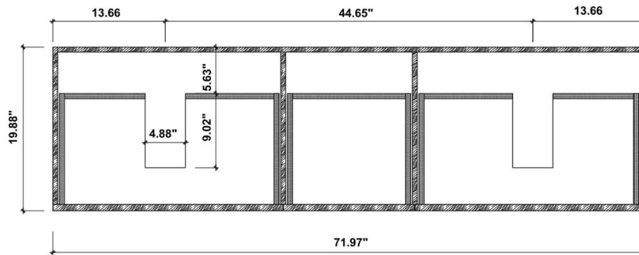
DRAWER PLAN DETAIL
