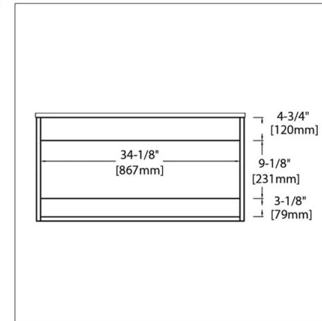
VANITY BACK
