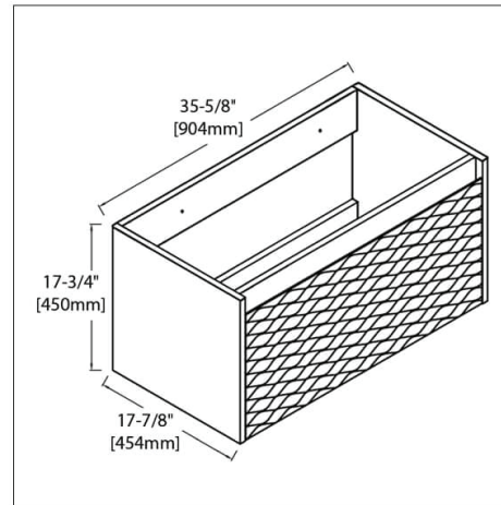
VANITY FRONT
