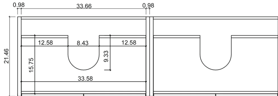
DRAWER PLAN DETAIL
