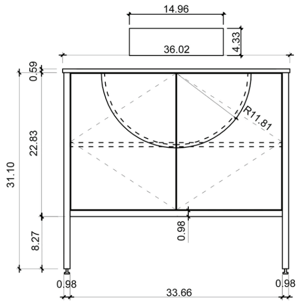
FRONT ELEVATION
