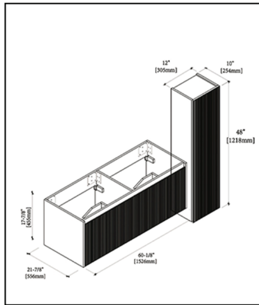
VANITY FRONT
