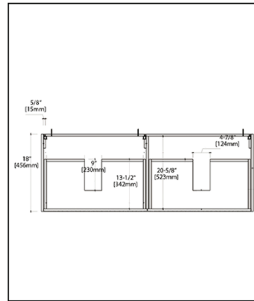
VANITY TOP
