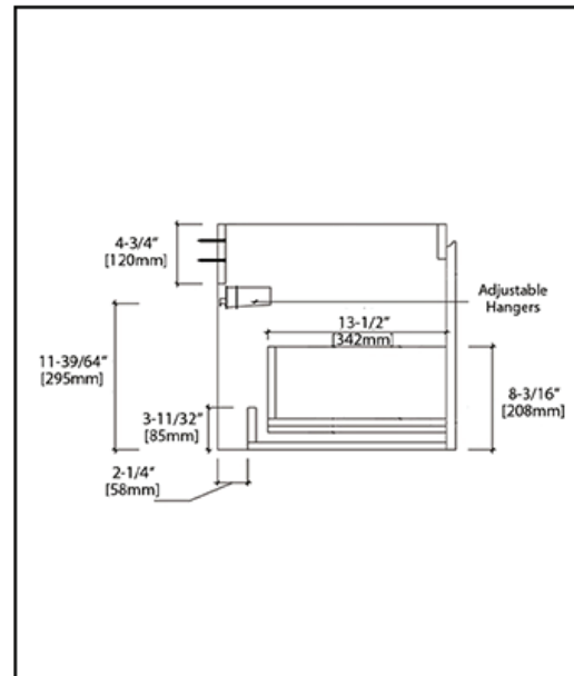
VANITY SIDE
