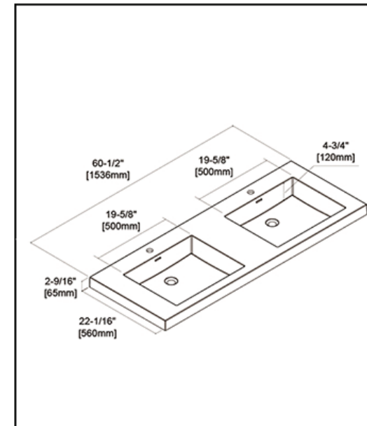
ACRYLIC SINK
