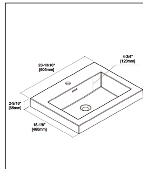
ACRYLIC SINK
