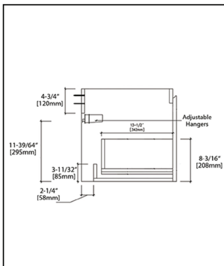
VANITY SIDE
