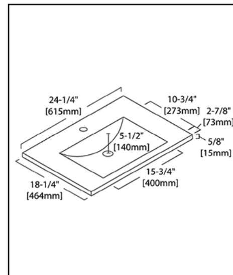
CERAMIC SINK
