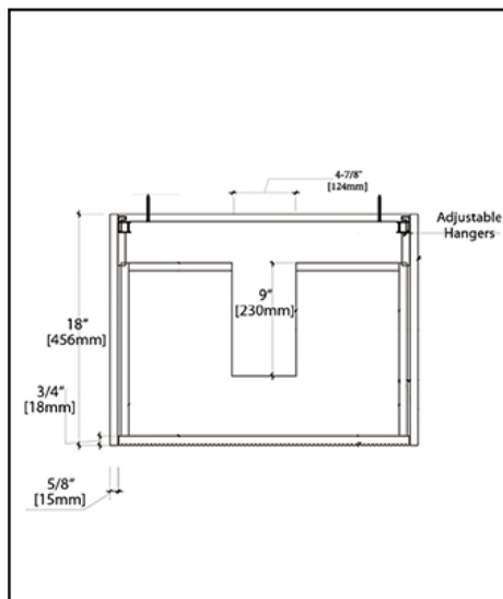
VANITY TOP
