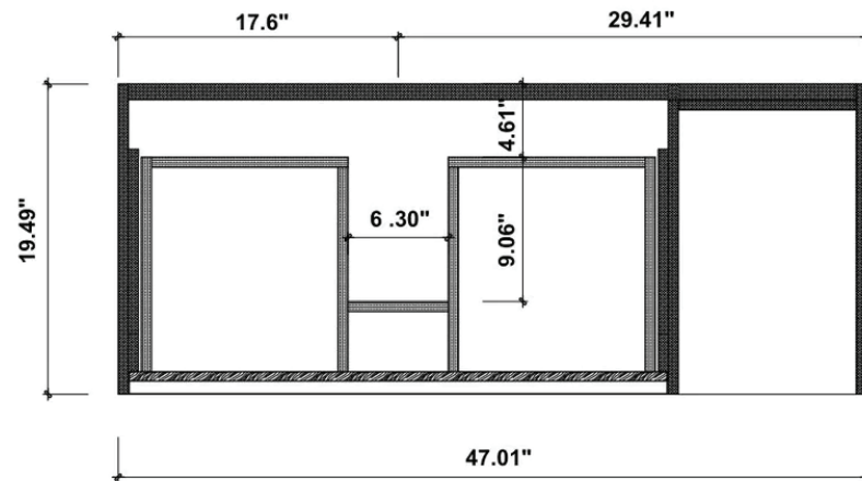
DRAWER PLAN DETAIL
