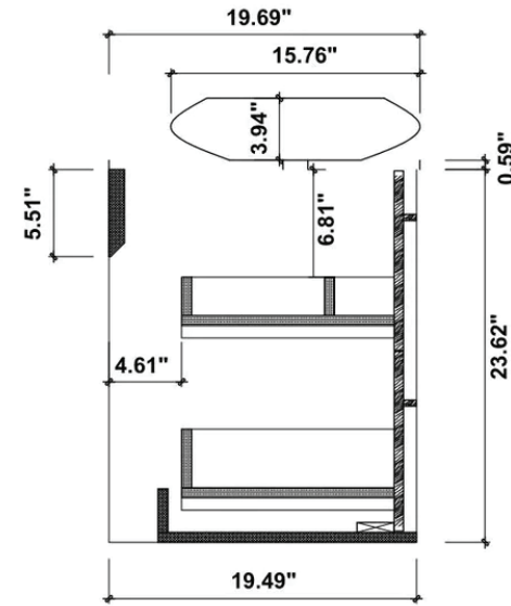
SIDE ELEVATION
