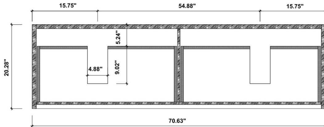
DRAWER PLAN DETAIL
