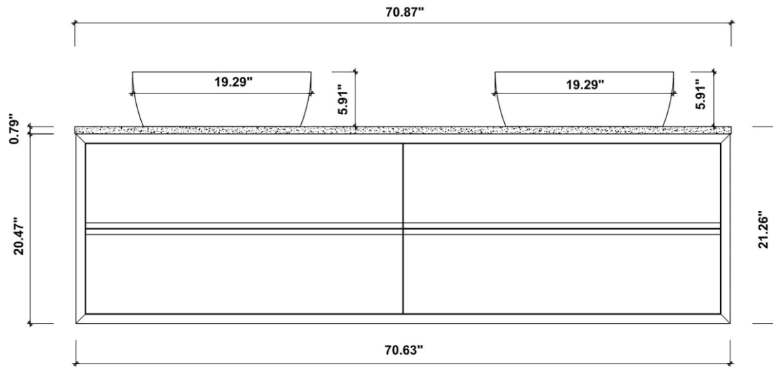
FRONT ELEVATION
