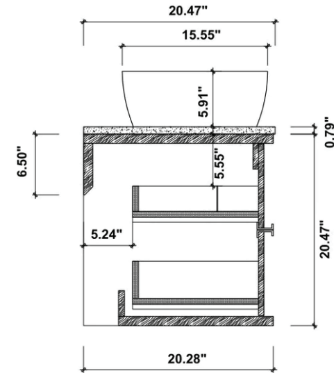
SIDE ELEVATION
