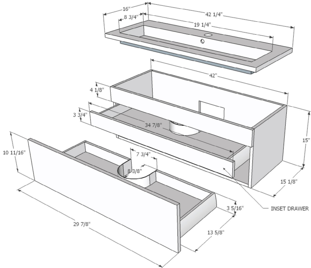
SINK DETAIL
