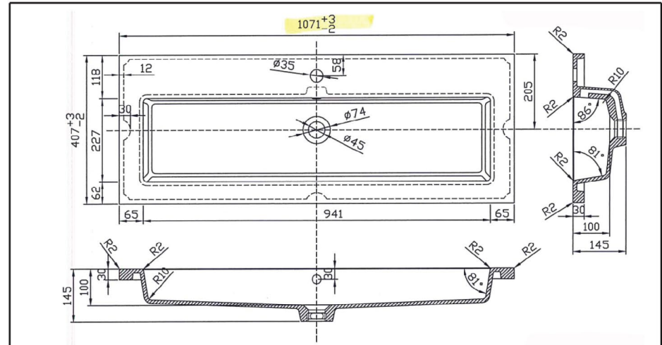
SINK DETAIL
