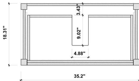
DRAWER PLAN DETAIL
