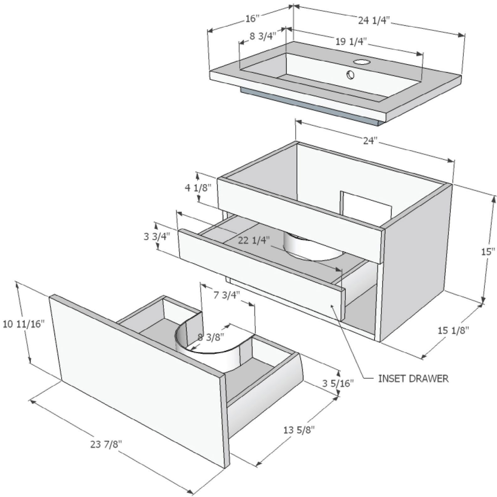
SINK DETAIL
