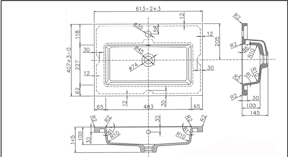
SINK DETAIL
