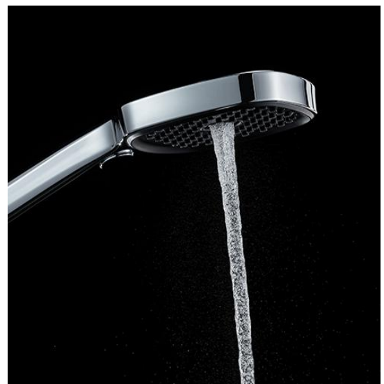
Scene Graph
