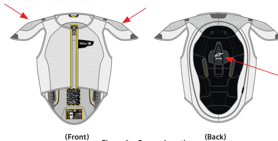
Figure 1 – Sensor Locations
