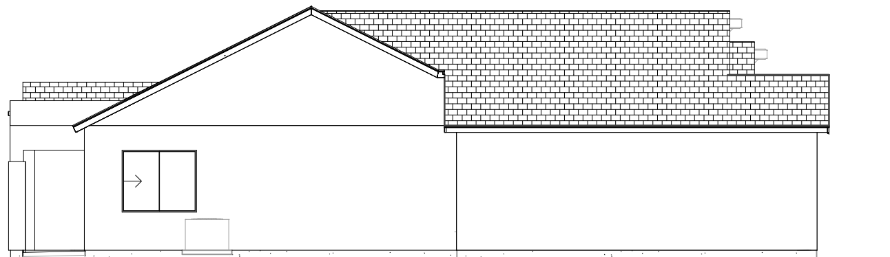
LEFT ELEVATION
