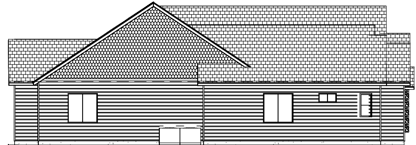
LEFT ELEVATION
