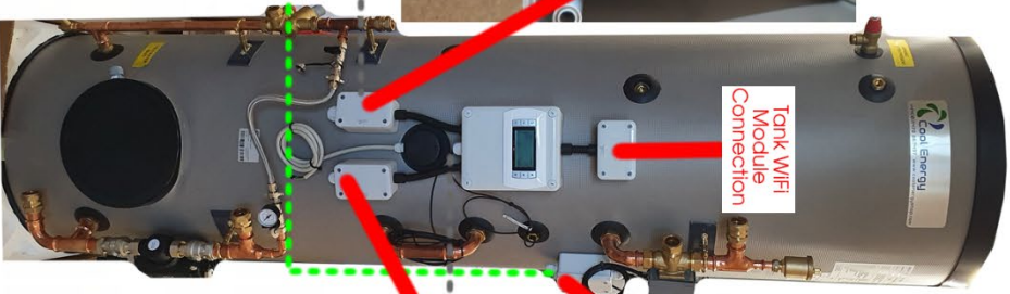
Buffer Tank
