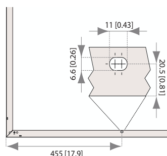
Fig. 15: Mounting holes
