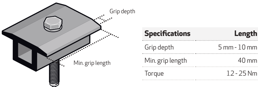
Fig. 1: Clamp specifications
