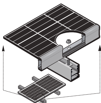
Fig. 17: Mounting hole installation example
