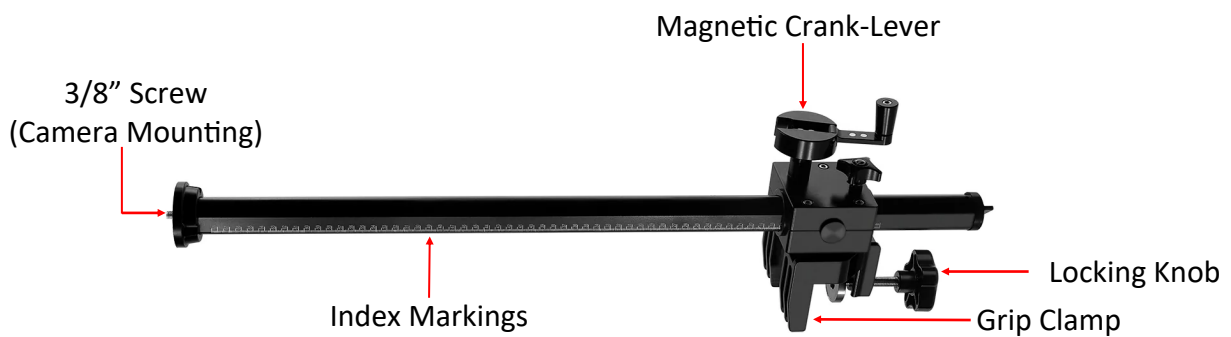
Proaim Tablemount Geared Column
