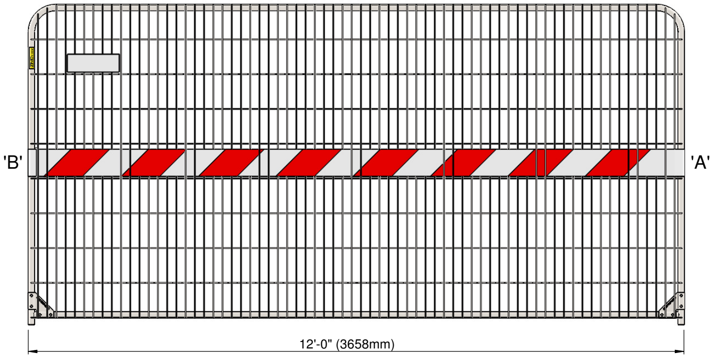
12'-0" (3658mm) VIEW ON FRONT FACE
