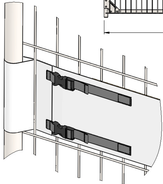
VIEW ON REAR FACE AT 'A'
