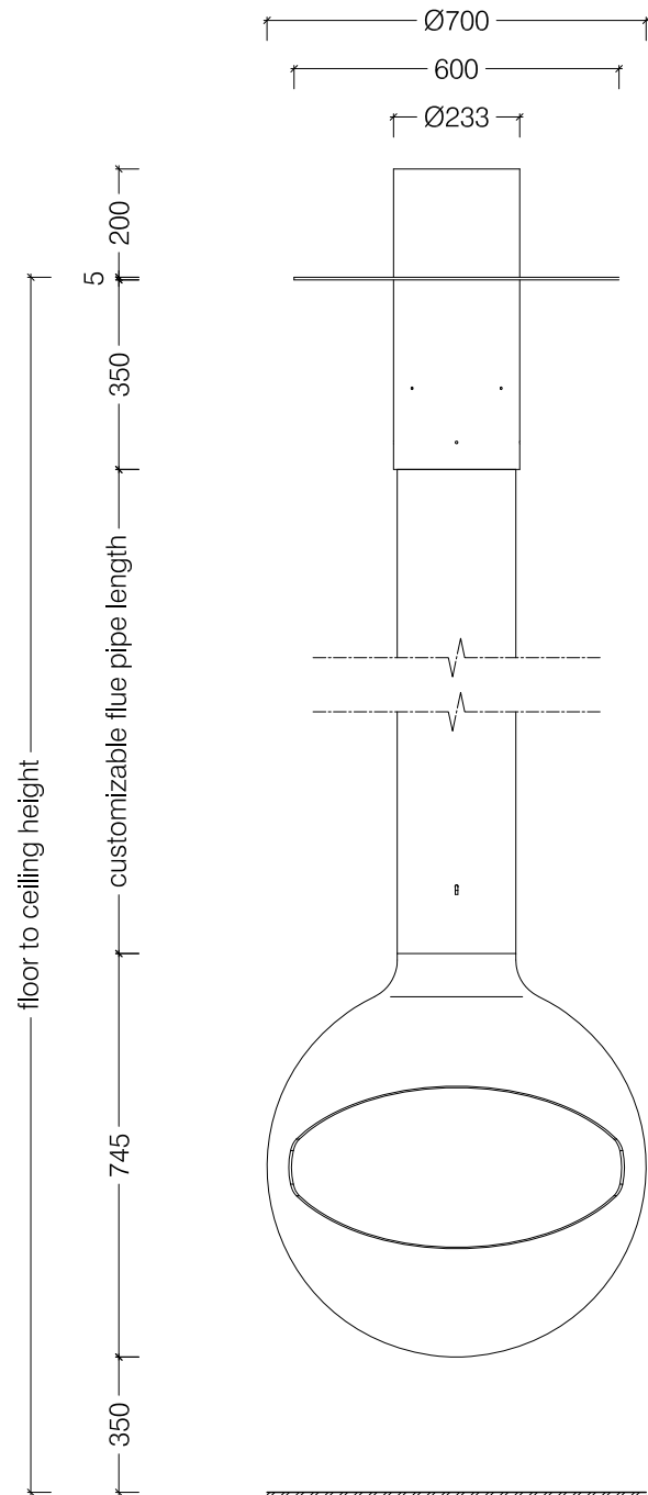
Front View
