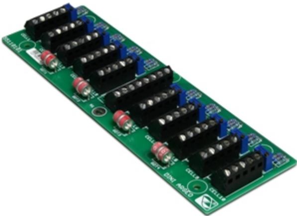
JC10Q: Junction and equalisation card with 10 inputs.
