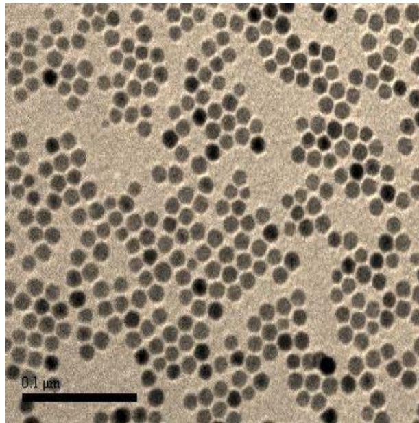
10nm Iron Oxide in Water
