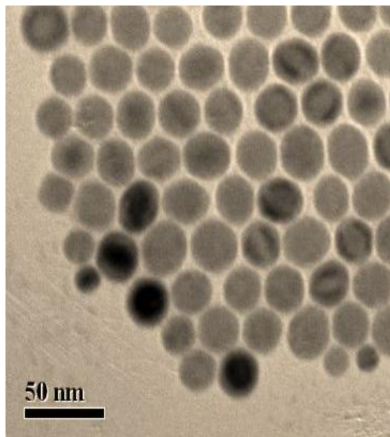
30nm Iron Oxide in Water
