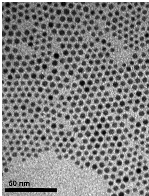
5nm Iron Oxide in Organic Solvent
