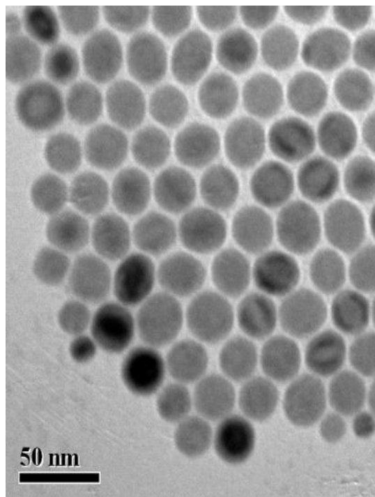
30nm Iron Oxide in Organic Solvent
