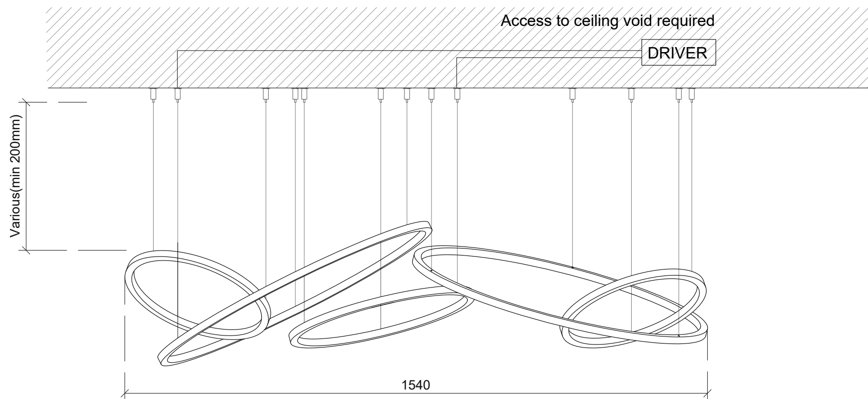
01-Elevation-Front View
