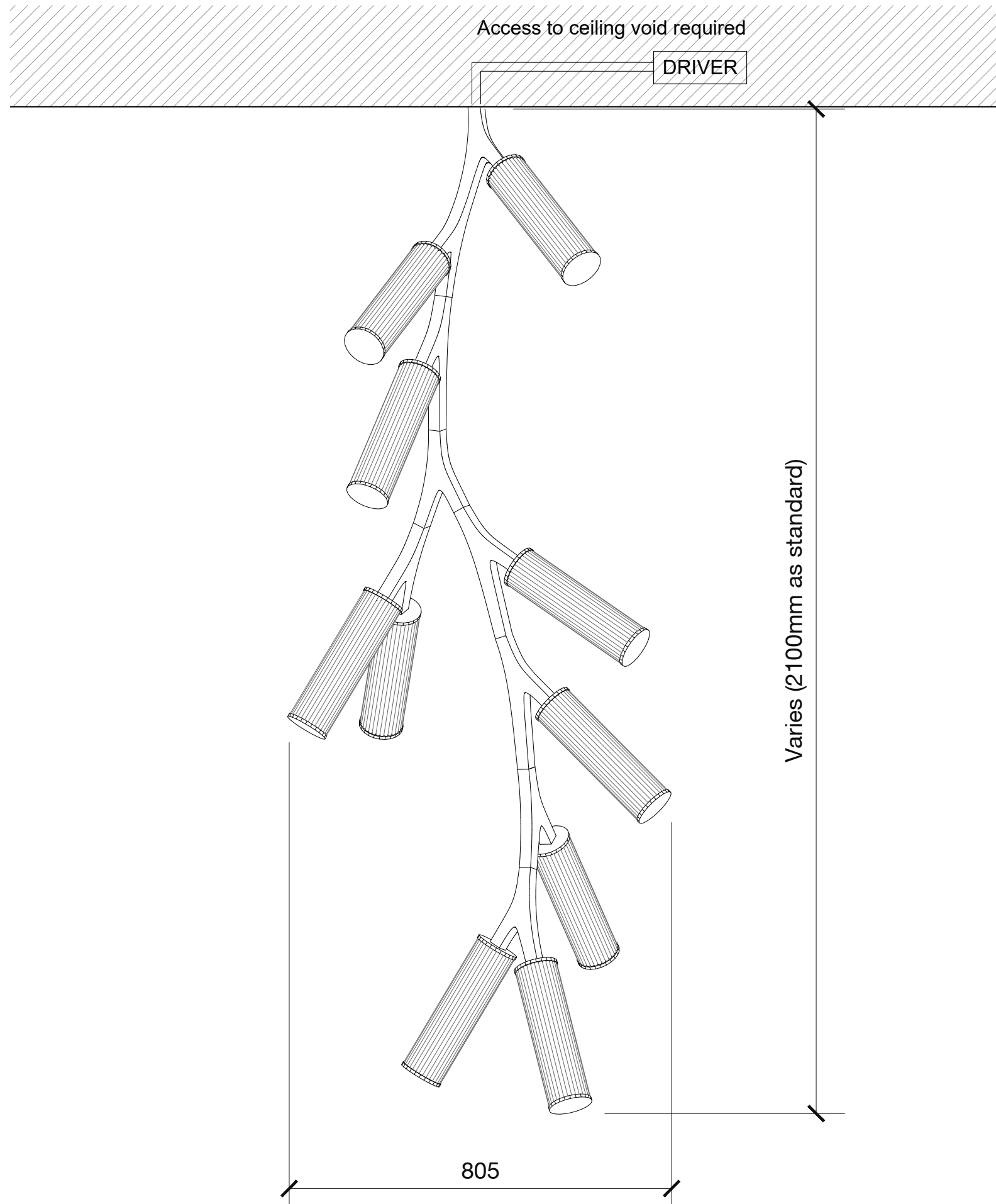
01-Haara Metsa Elevation View
