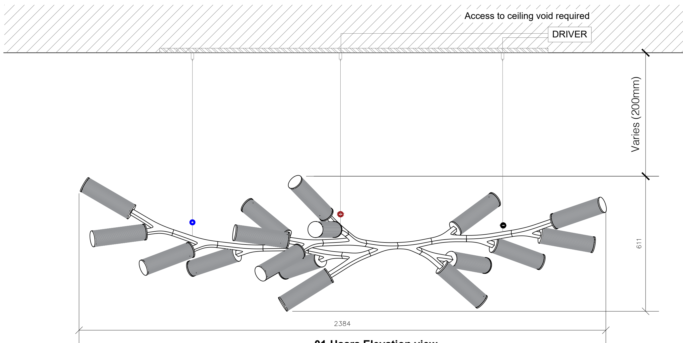
01-Haara Elevation view
