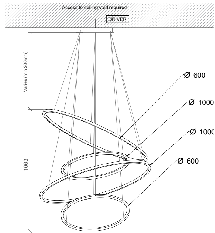
Lohja Elevation View
