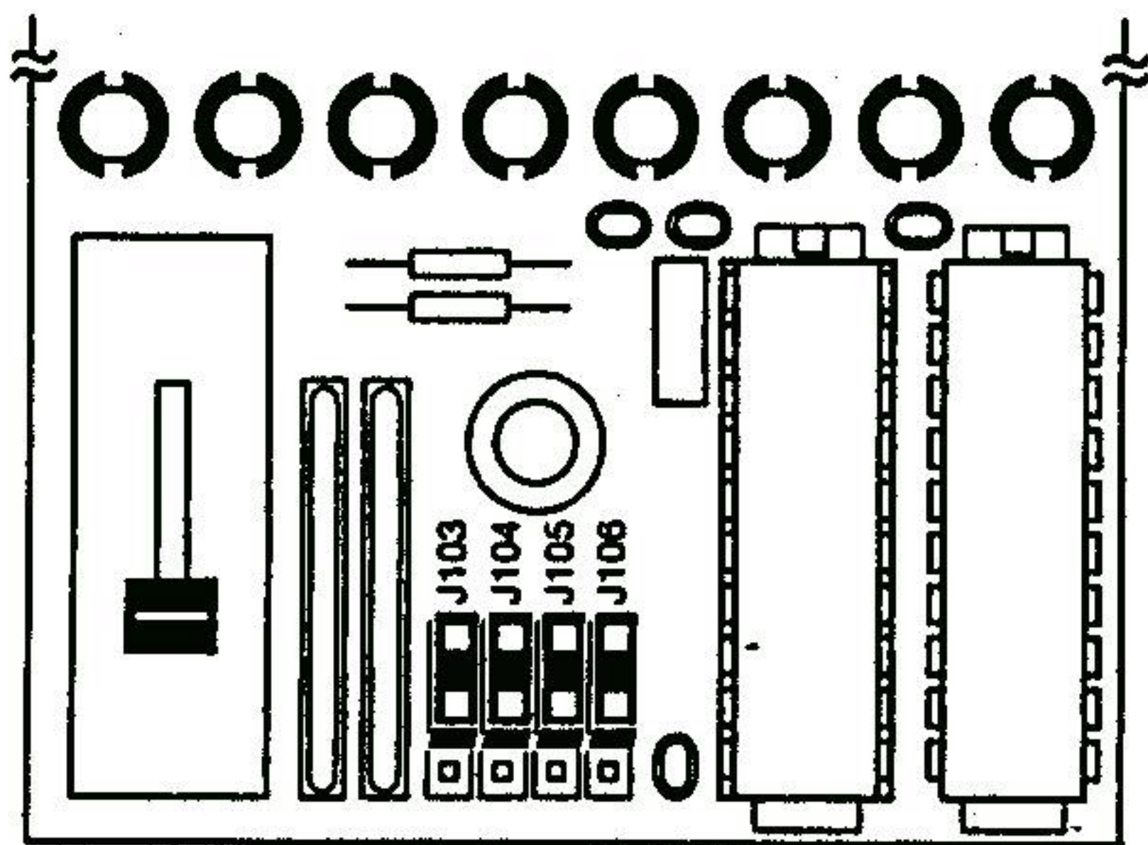
USER PROGRAMMABLE JUMPER DIAGRAM
