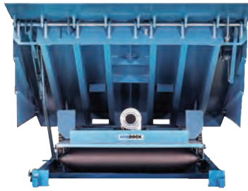
Air-Powered Levelers
