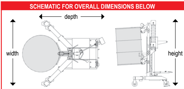
Power Lift
