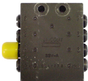
SSV Divider Valve with 8 Outlets & Indicator Pin
