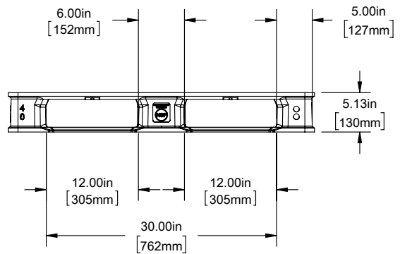
SIDE VIEW - 40"
