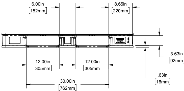
SIDE VIEW - 48"
