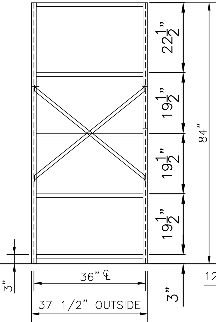
FRONT VIEW Shelves are adjustable on 1-1/2" Centers 36" X 84"
