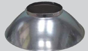
HBBR-480 Aluminum reflector for LED-E40-90W ø480 x H140mm
