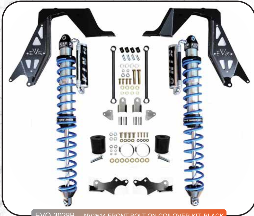
EVO-3028B NV2514 FRONT BOLT-ON COILOVER KIT, BLACK
