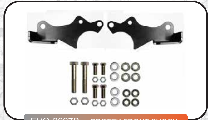
EVO-3027B PROTEK FRONT SHOCK RELOCATION BRACKETS
