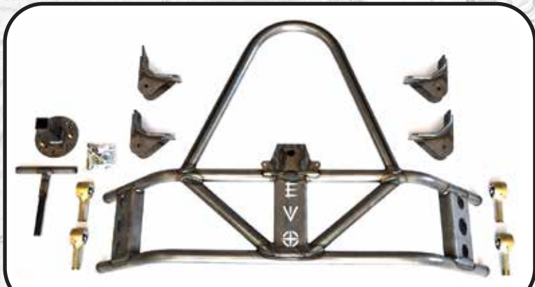
EVO-1069 REAR TIRE CARRIER CAGE
