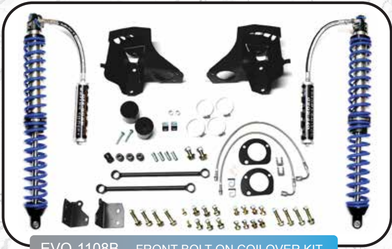
EVO-1108B FRONT BOLT ON COILOVER KIT
