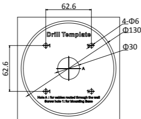
Figure 2-12 Drill Template
