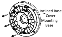
Figure 2-18 Fix Camera's Mounting Base
