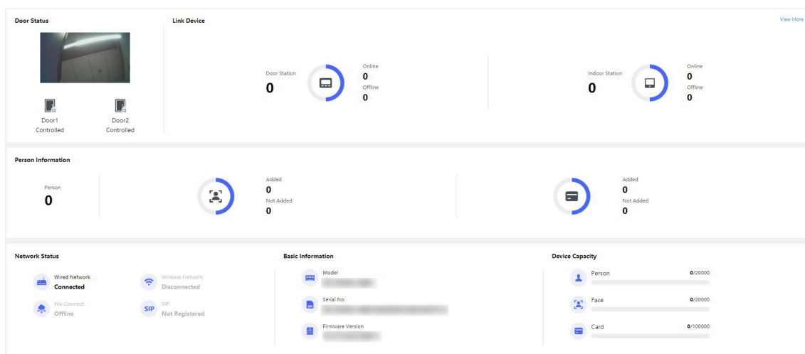
Figure 8-1 Overview Page
