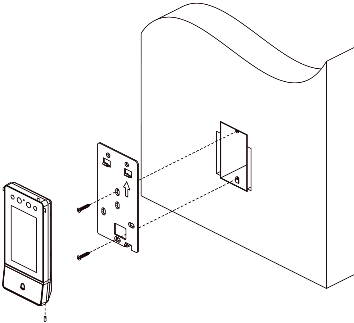
Figure 3-4 Flush Mounting
