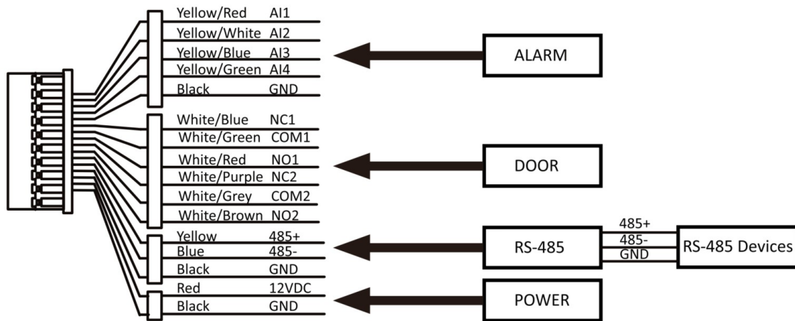
Figure 2-1 Terminal Description
