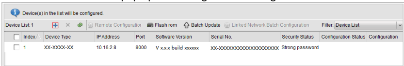
Figure 3-7 Adding Button
