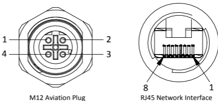
Figure 1-3 RJ45 Interface and M12 Aviation Plug
