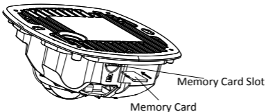
Figure 2-2 Install the Memory Card
