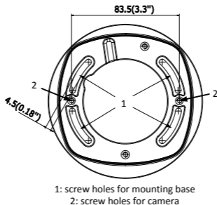
Figure 2-5 Screw Holes on Mounting Base
