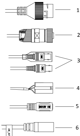
Figure 1-2 Cable Overview
