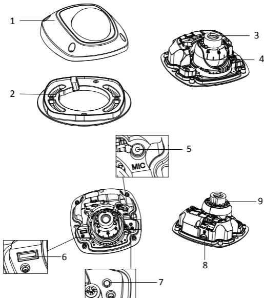
Figure 1-1 Overview of Mobile Network Mini Dome Camera
