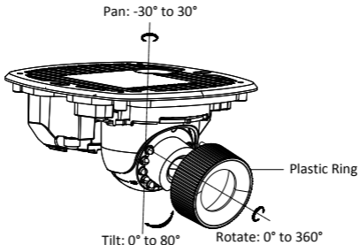
Figure 2-8 3-Axis Adjustment
