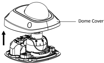
Figure 2-1 Disassemble the Camera
