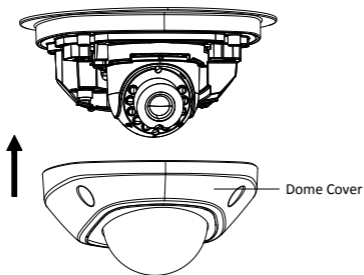
Figure 2-9 Install the Dome Cover
