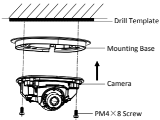
Figure 2-7 Fix the Camera
