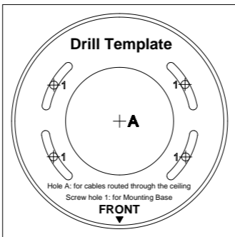
Figure 2-3 Drill Template
