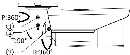
Figure 2-3 3-axis Adjustment
