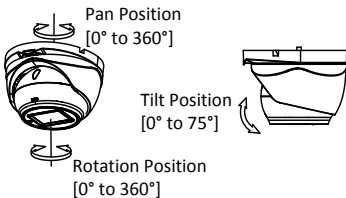
Figure 2-12 3-axis Adjustment
