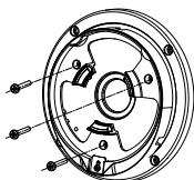
Figure 2-14 Secure Screws on Junction Box's Cover
