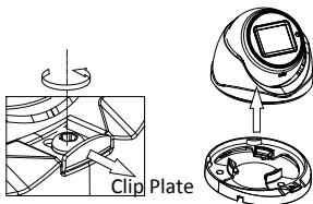
Figure 2-9 Remove the Clip Plate
