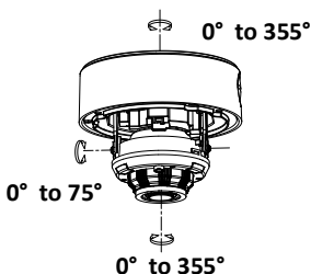
Figure 2-4 3-Axis Adjustment
