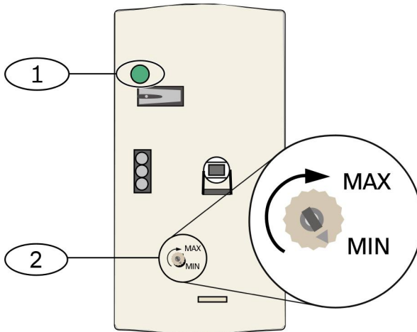
Figure 6.1: Sensitivity settings
