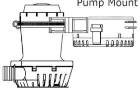
BG-SW mounted to the pump
