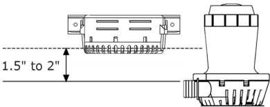
Mount BG-SW horizontally 1.5" - 2.0" above pump outlet
