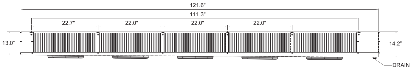
FRONT VIEW
