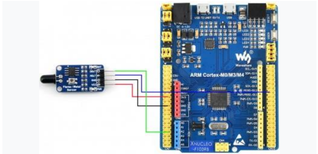
Hardware connection-STM32
