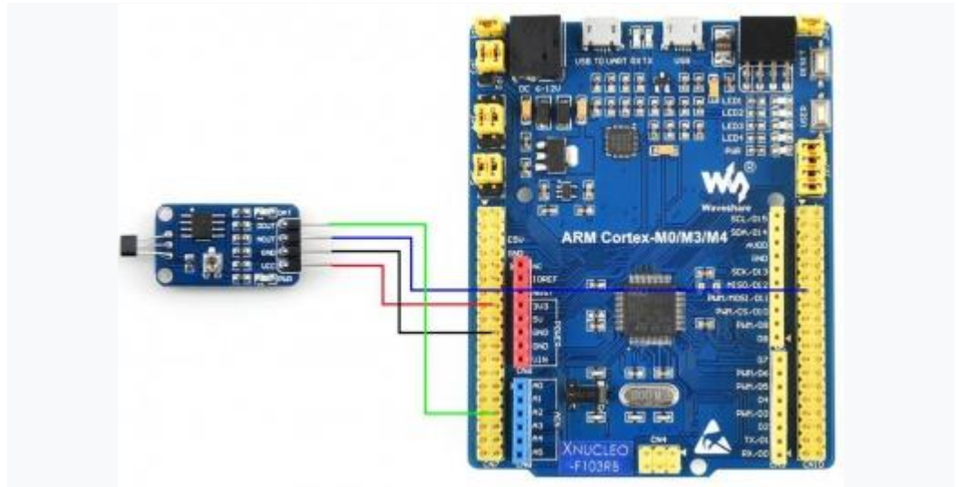
Hardware connection-STM32
